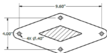
FOOT MOUNT
